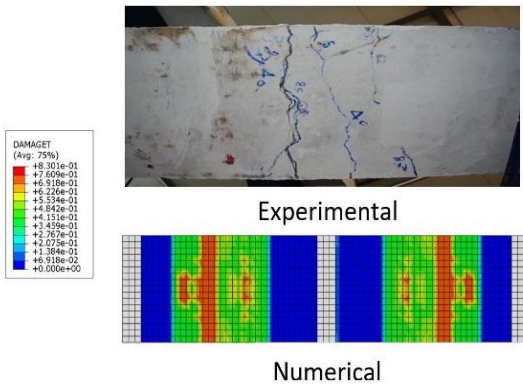
Figure 12: Experimental and Numerical Cracks Pattern of S-O-4 specimen
