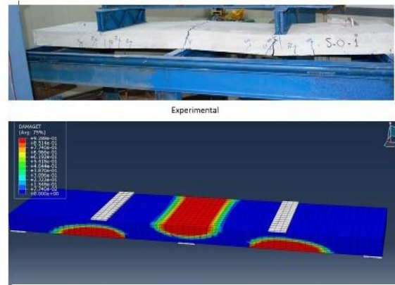
Figure 15: Failure Mode of S-O-1 Specimen
