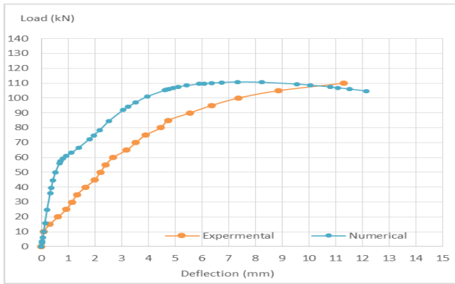
Figure 5: Experimental and Numerical Load-Deflection Curves for S-O-1 Specimen
