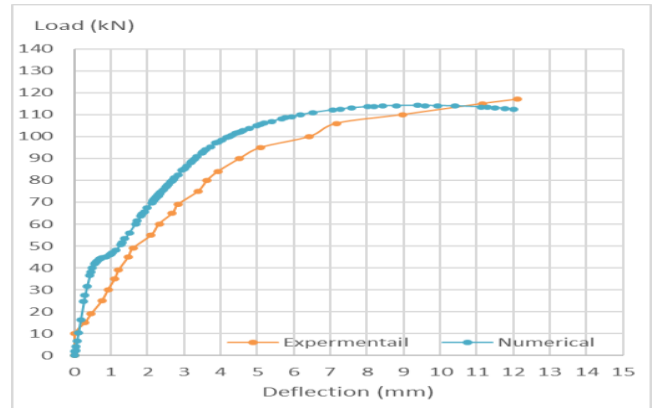
Figure 8: Experimental and Numerical Load-Deflection Curves for S-O-5 Specimen
