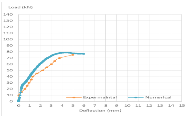
Figure 6: Experimental and Numerical Load-Deflection Curves for S-O-2 and S-O-3 Specimens
