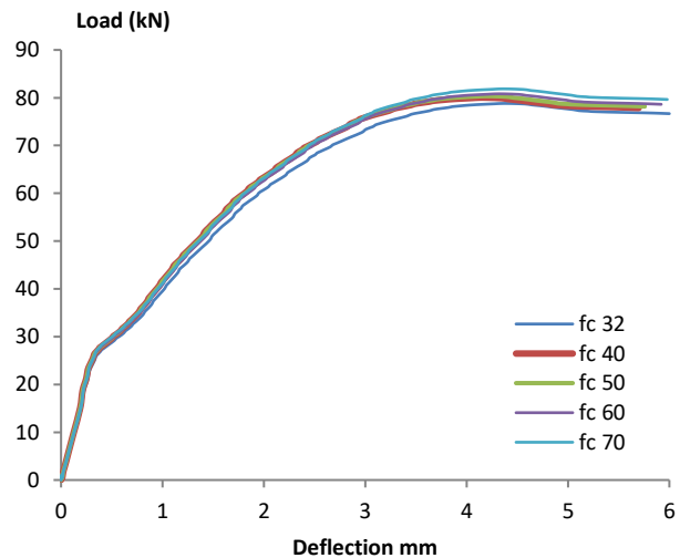
Figure 25: Load-Deflection Curves for Parametric Study
