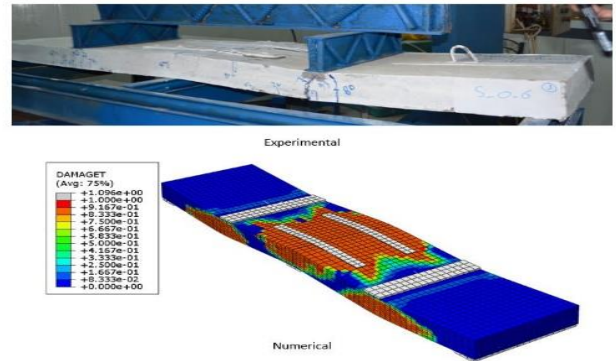
Figure 19: Failure Mode of S-O-6 Specimen
