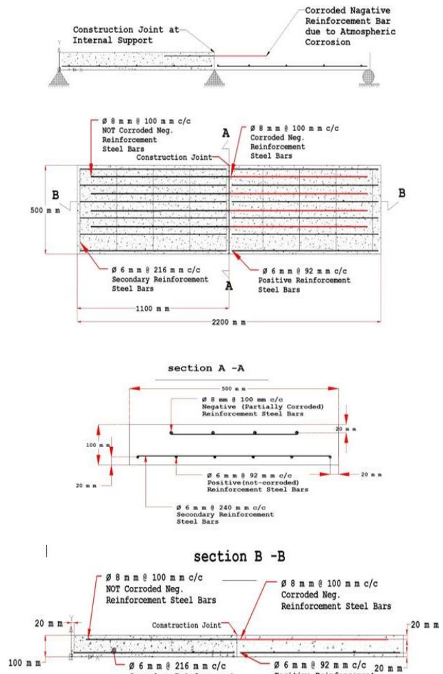
Figure 1: Specimens Dimension and Reinforcement Details [12]
