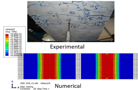
Figure 14: Experimental and Numerical Cracks Pattern of S-O-6 specimen
