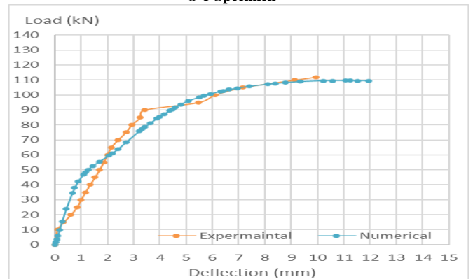
Figure 9: Experimental and Numerical Load-Deflection Curves for S-O-6
