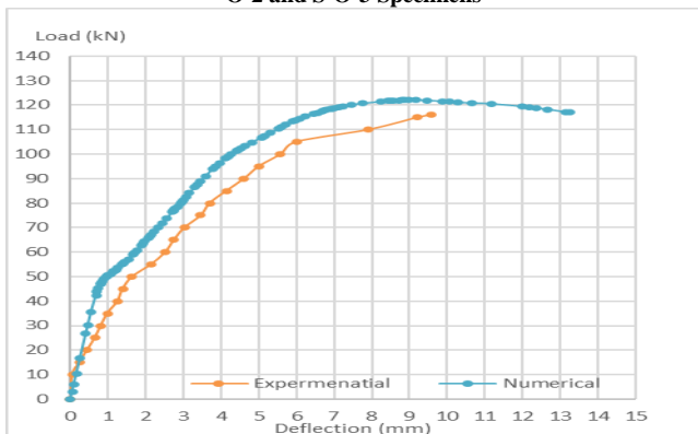
Figure 7: Experimental and Numerical Load-Deflection Curves for S-O-4 specimen
