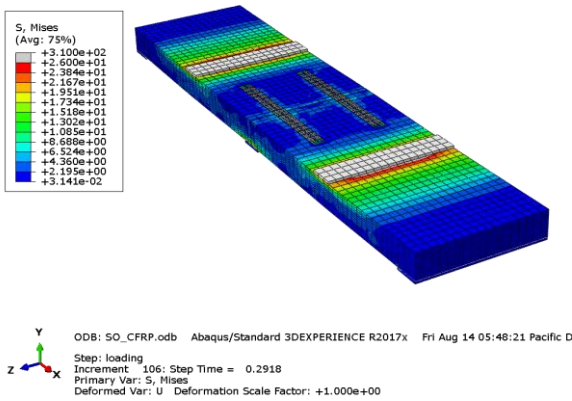
Figure 22: Mises Stresses in S-O-4 Specimen
