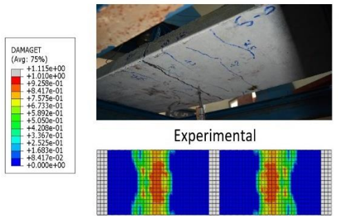
Figure 11: Experimental and Numerical Cracks Pattern of S-O-3 specimens
