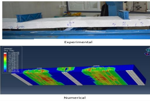
Figure 17: Failure Mode of S-O-2 and S-O-3 Specimens
