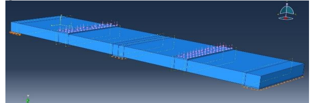
Figure 4: Loading and Boundary Conditions
