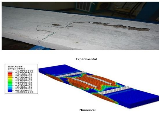
Figure 16: Failure Mode of S-O-4 Specimen
