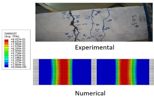
Figure 13: Experimental and Numerical Cracks Pattern of S-O-5 specimen
