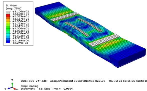
Figure 24: Mises Stresses in S-O-6 Specimen
