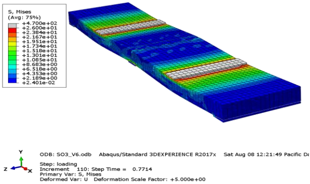
Figure 21: : Mises Stresses in S-O-2 and S-O-3SpecimenS
