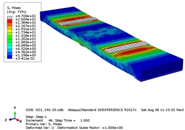
Figure 20: Mises Stresses in S-O-1 Specimen
