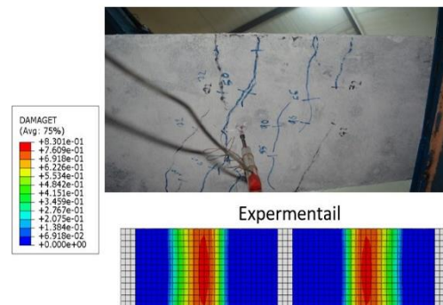
Figure 10: Experimental and Numerical Cracks Pattern of S-O-1 specimen
