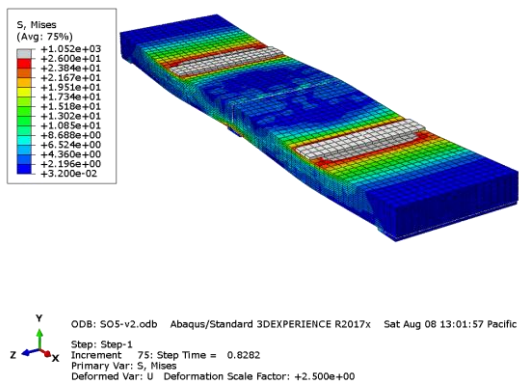
Figure 23: Mises Stresses in S-O-5 Specimen
