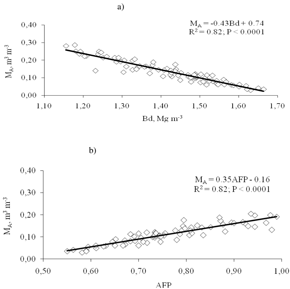
Figure 2. Relationship between (a) macroporosity ( M_A ) and bulk density ( \text{Bd} ) and (b) M_A and air-filled porosity ( \text{AFP} ) of an Alfisol to 0.00 – 0.20 m depth.
