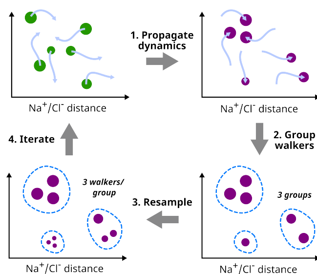
Figure 13. Flow chart for simulating Na + /Cl - association using the new binless resampler module. After dynamics propagation in step 1, trajectories in each bin are grouped with the user-specified group.py function. In this example, trajectory walkers are grouped using k-means clustering.
