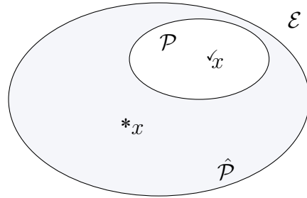
Figure 1: Positional licensing
